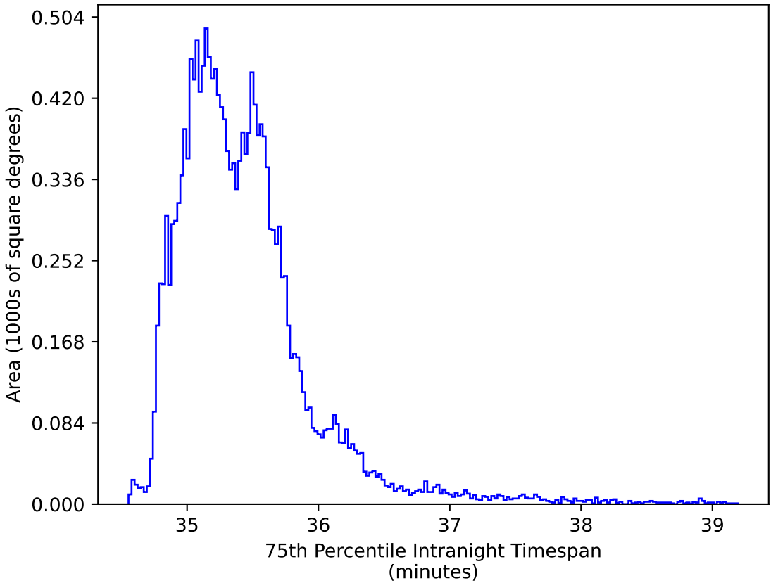
internal_u_expt45_nscale0.9v3.4_10yrs WFD: 75th Percentile Intranight Timespan
