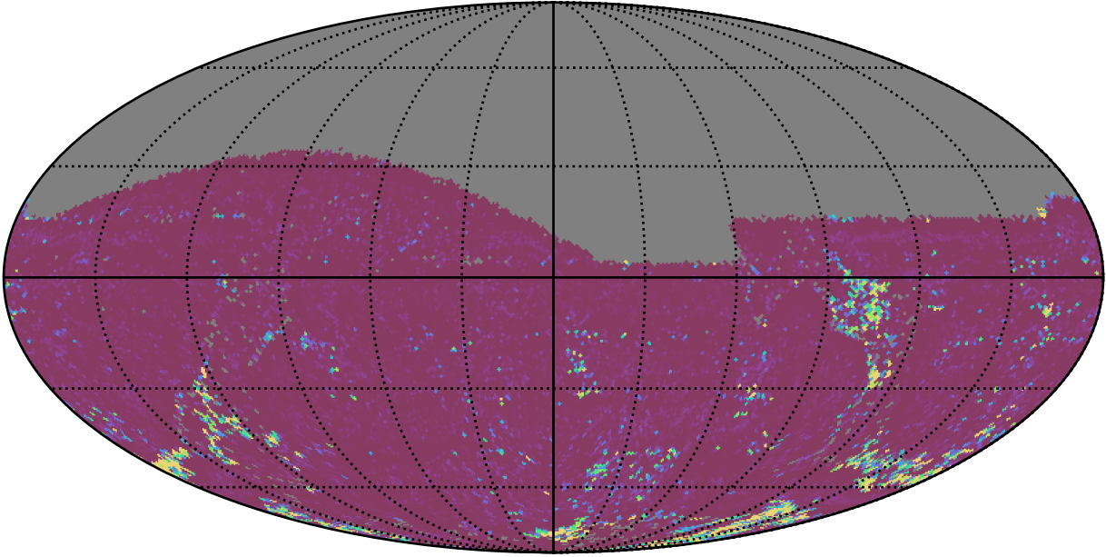
internal_u_expt45_nscale0.9v3.4_10yrs All sky g band: 75th Percentile Intranight Timespan
