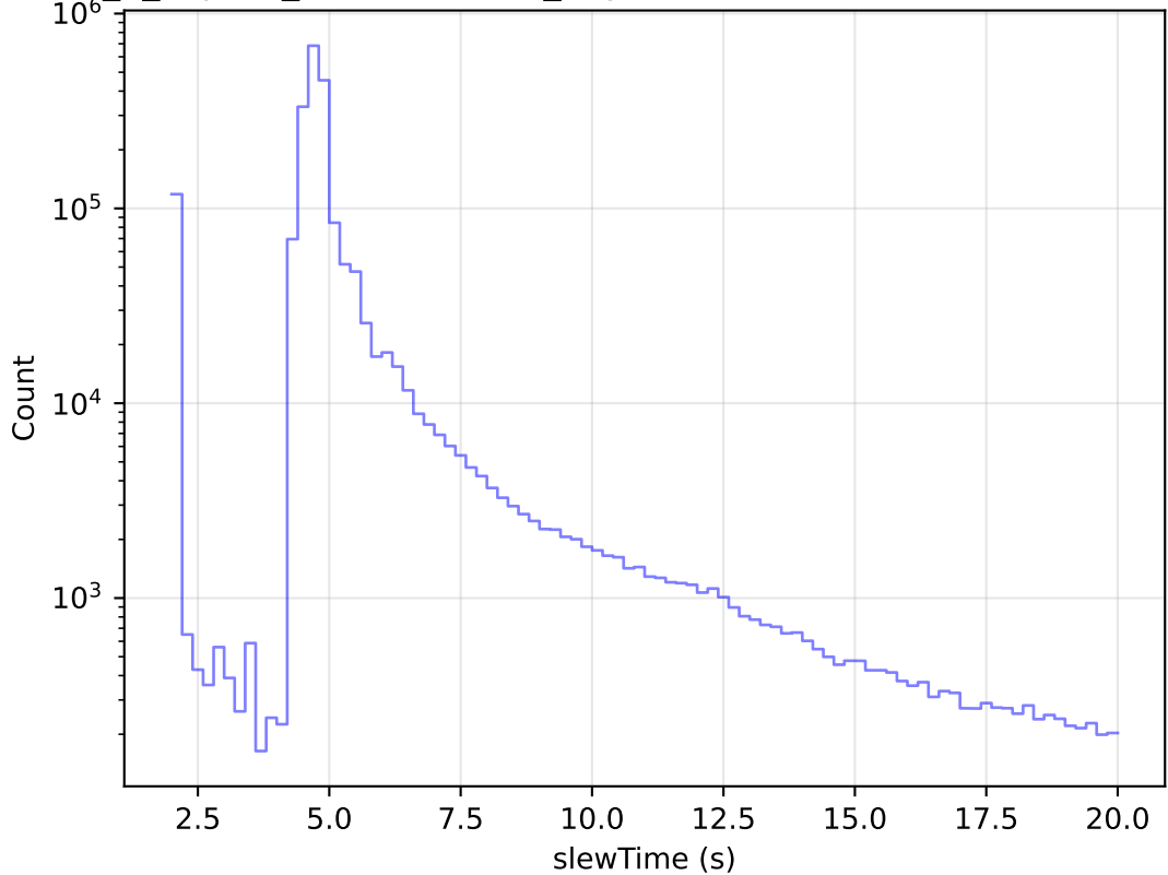
internal_u_expt45_nscale0.9v3.4_10yrs All visits: Zoom Slew Time Histogram
