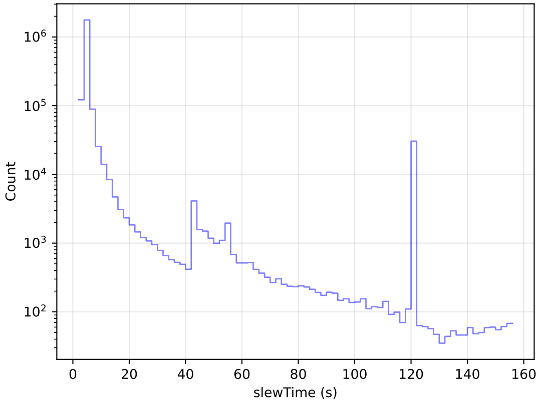
internal_u_expt45_nscale0.9v3.4_10yrs All visits: Slew Time Histogram
