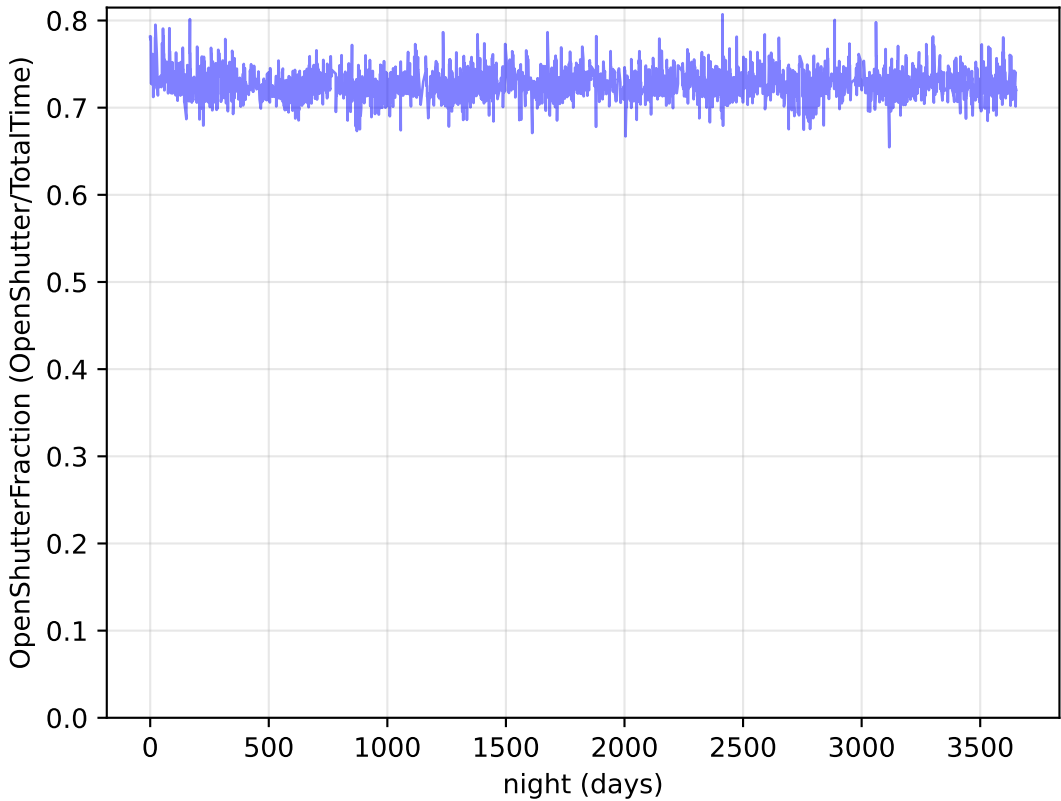
internal_u_expt45_nscale0.9v3.4_10yrs : OpenShutterFraction
