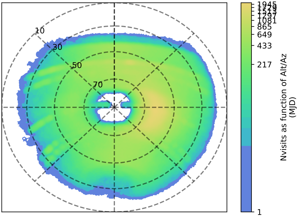
internal_u_expt45_nscale0.9v3.4_10yrs y: Nvisits as function of Alt/Az
