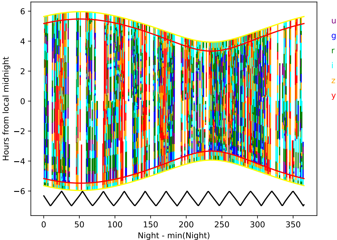
internal_u_expt45_nscale0.9v3.4_10yrs year 7-8: Hourglass
