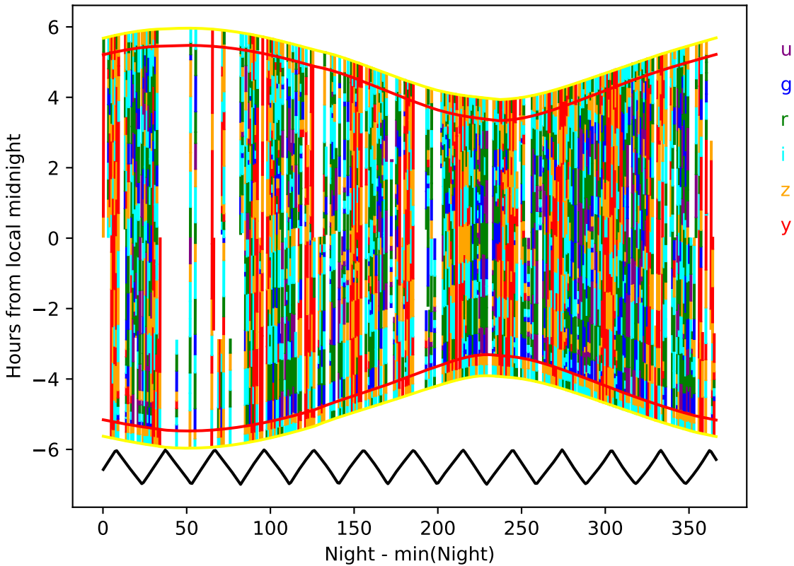
internal_u_expt45_nscale0.9v3.4_10yrs year 3-4: Hourglass
