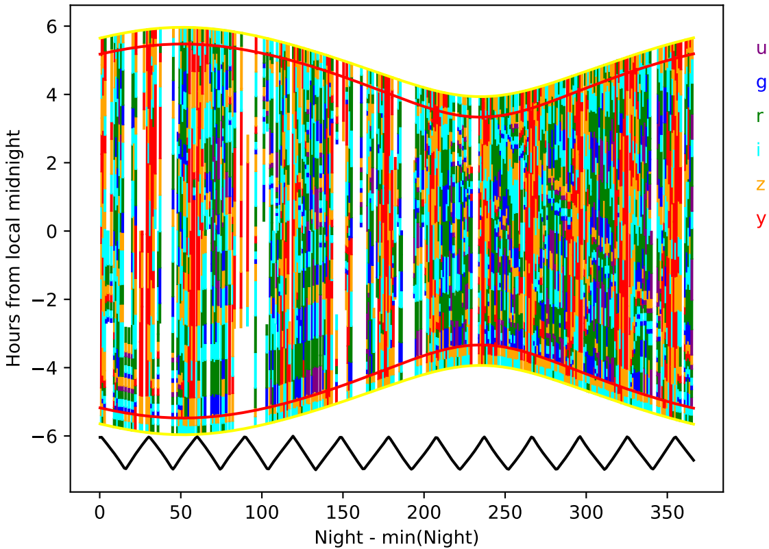
internal_u_expt45_nscale0.9v3.4_10yrs year 1-2: Hourglass
