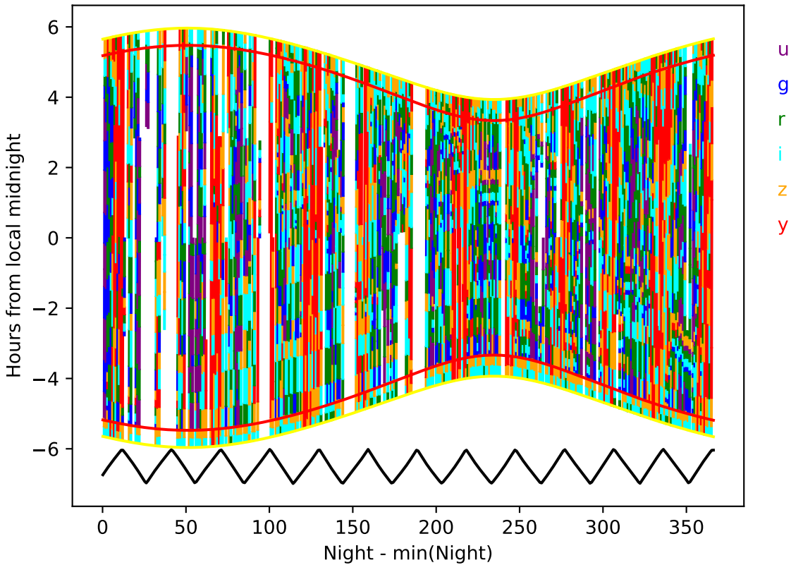
internal_u_expt45_nscale0.9v3.4_10yrs year 0-1: Hourglass
