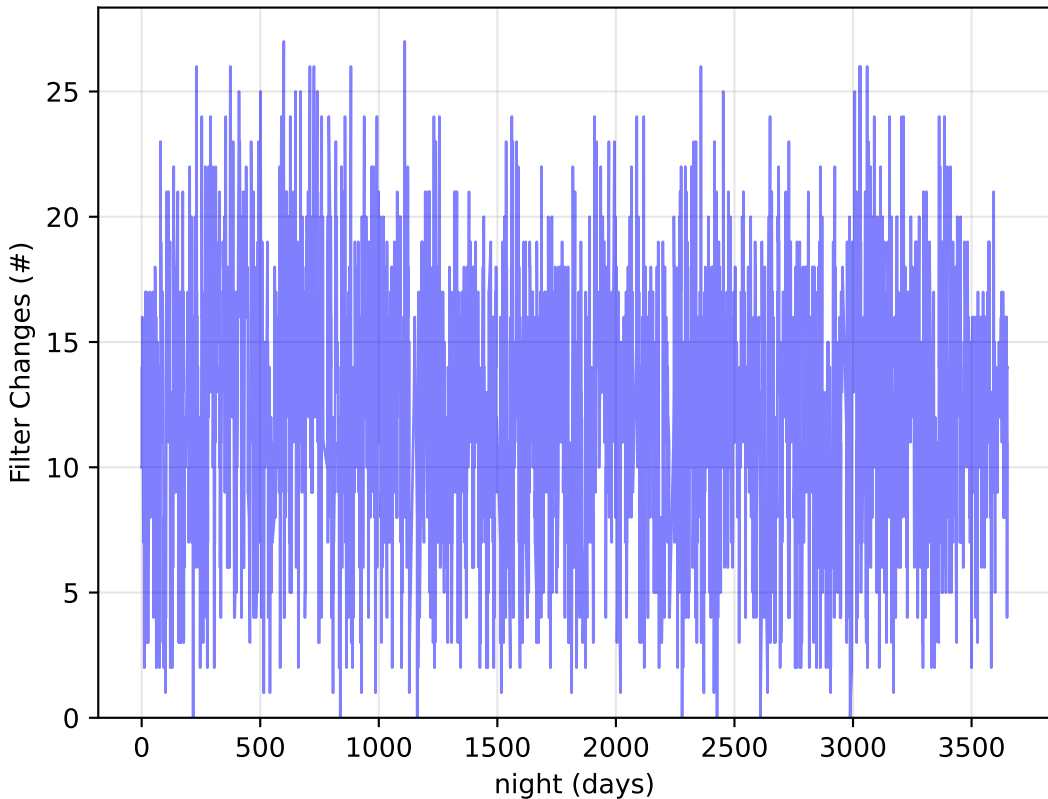
internal_u_expt45_nscale0.9v3.4_10yrs : Filter Changes
