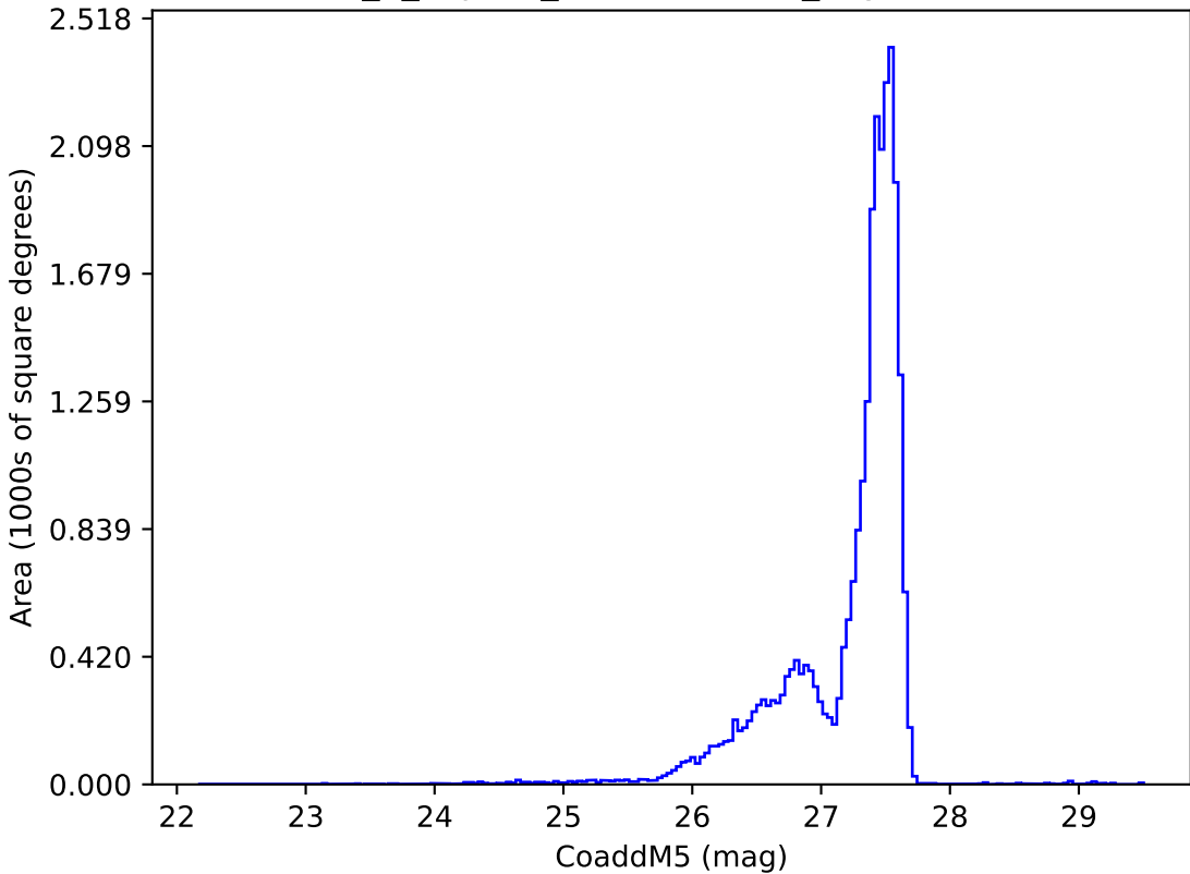
internal_u_expt45_nscale0.9v3.4_10yrs : CoaddM5
