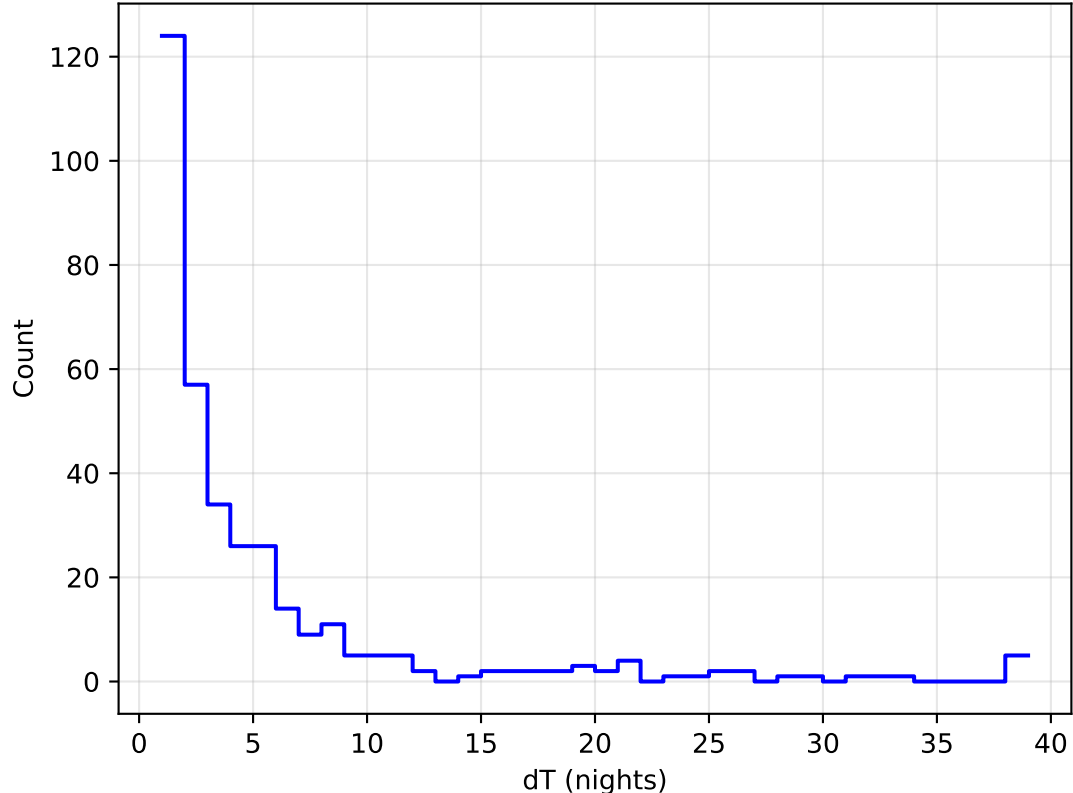
internal_u_expt45_nscale0.9v3.4_10yrs all bands: DD:WFD Delta Nights Histogram
