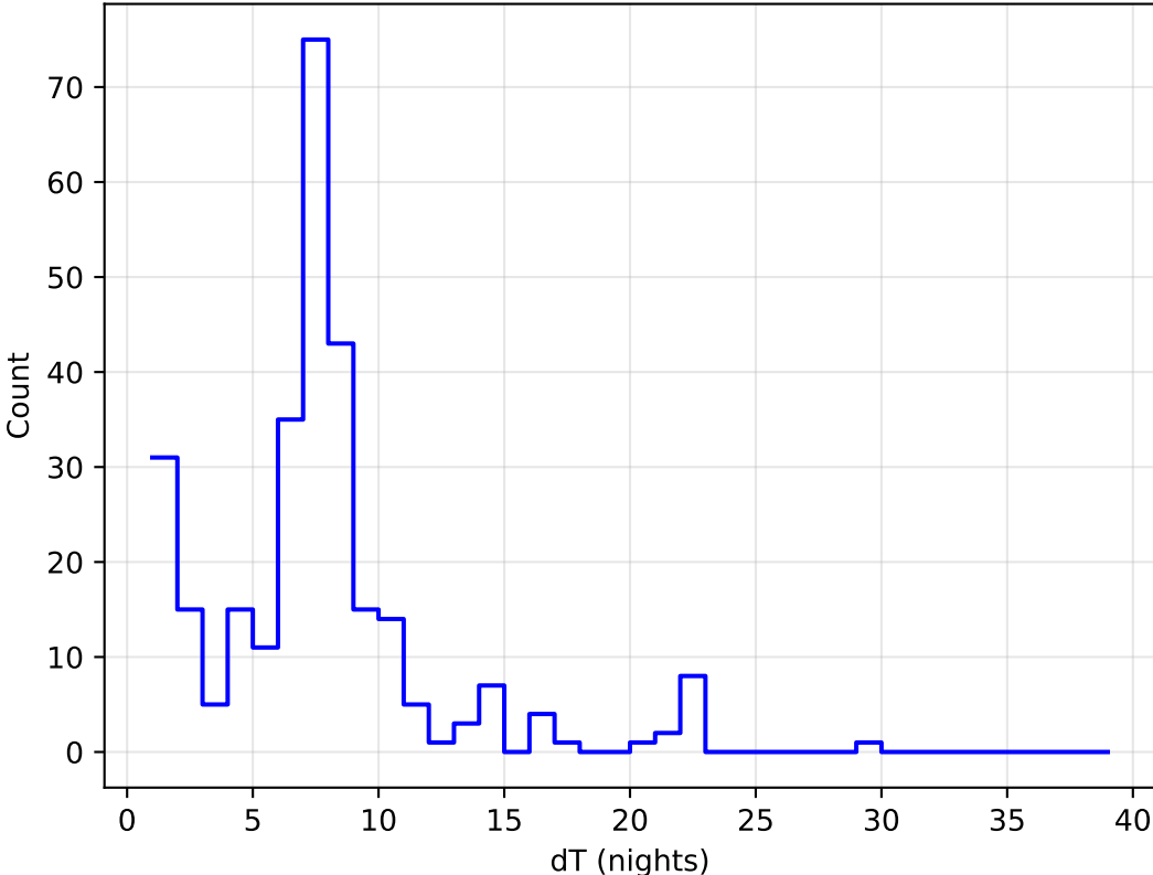
internal_u_expt45_nscale0.9v3.4_10yrs all bands: DD:EDFS Delta Nights Histogram
