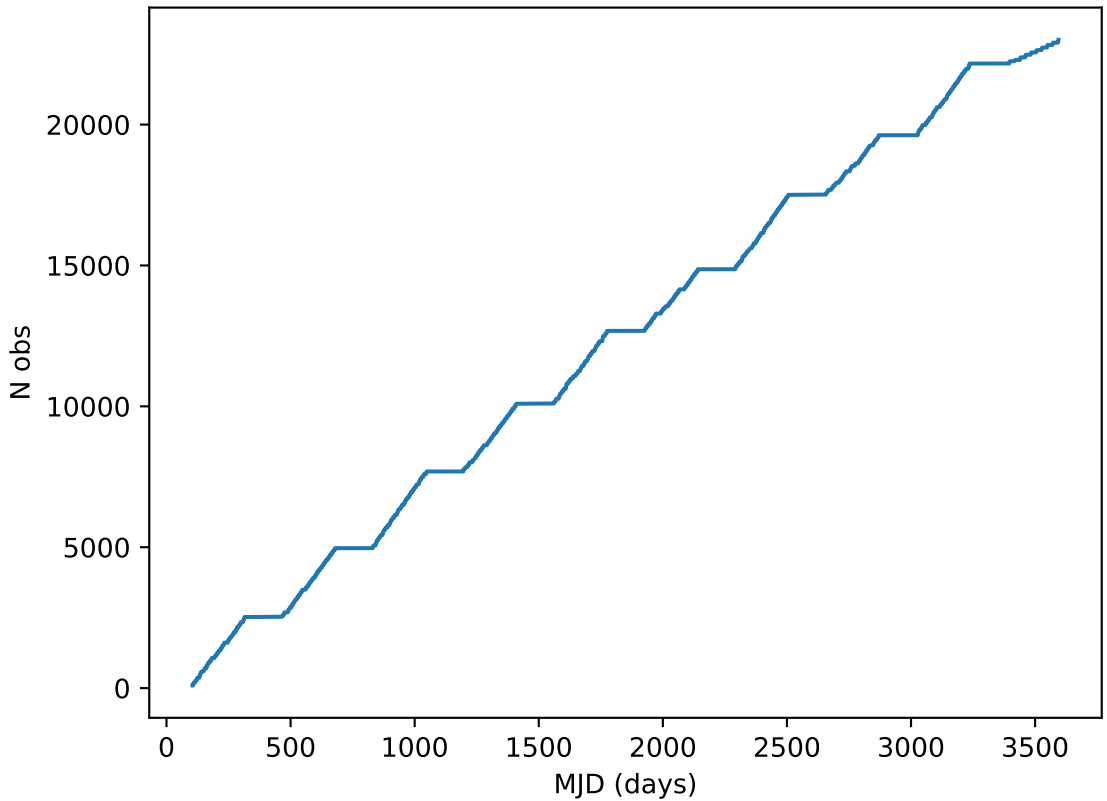
internal_u_expt45_nscale0.9v3.4_10yrs all bands: DD:EDFS Cumulative NVisits
