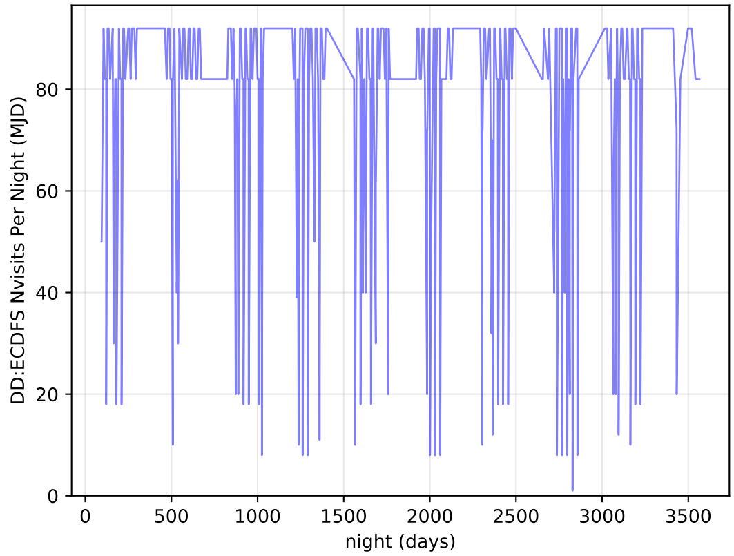
internal_u_expt45_nscale0.9v3.4_10yrs all bands: DD:ECDFS Nvisits Per Night
