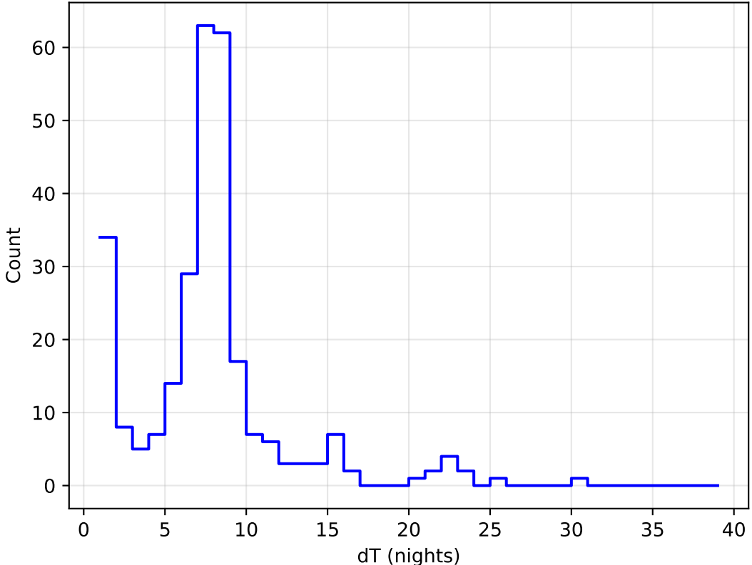
internal_u_expt45_nscale0.9v3.4_10yrs all bands: DD:ECDFS Delta Nights Histogram
