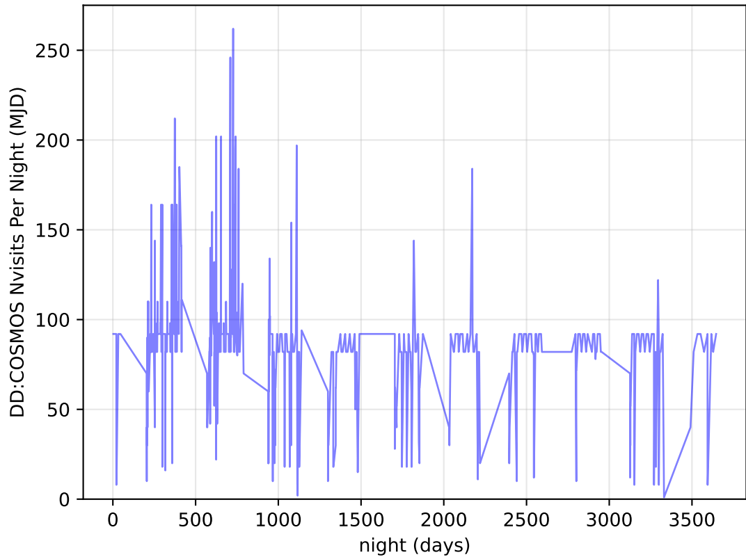
internal_u_expt45_nscale0.9v3.4_10yrs all bands: DD: COSMOS Nvisits Per Night
