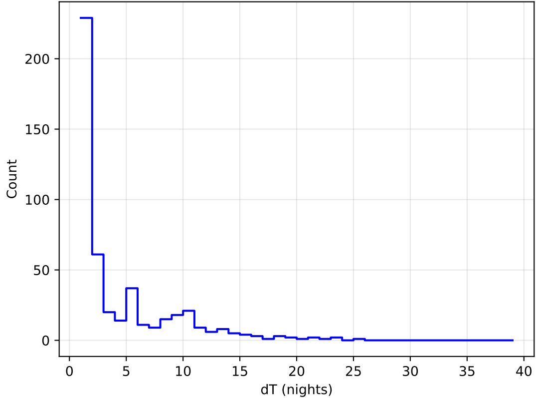
internal_u_expt45_nscale0.9v3.4_10yrs all bands: DD: COSMOS Delta Nights Histogram
