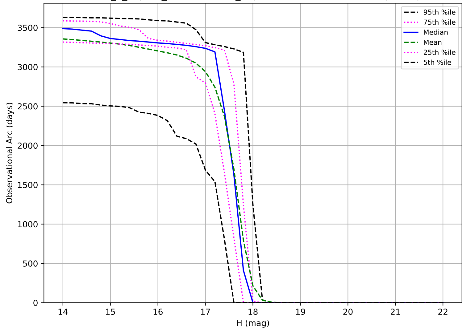
internal_u_expt38_nscale1.5v3.4_10yrs: Observational Arc Length Trojan
