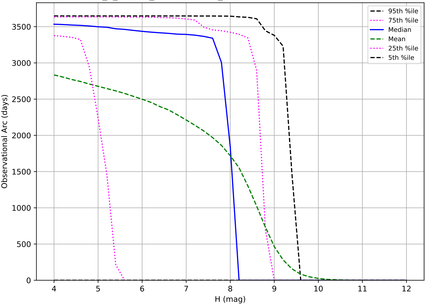
internal_u_expt38_nscale1.5v3.4_10yrs: Observational Arc Length TNO
