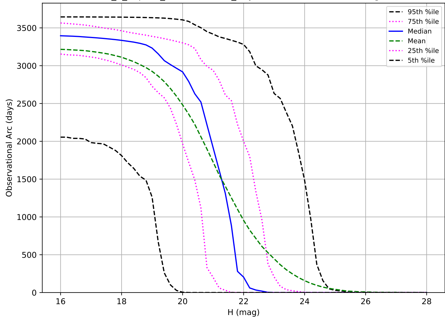
internal_u_expt38_nscale1.5v3.4_10yrs: Observational Arc Length PHA
