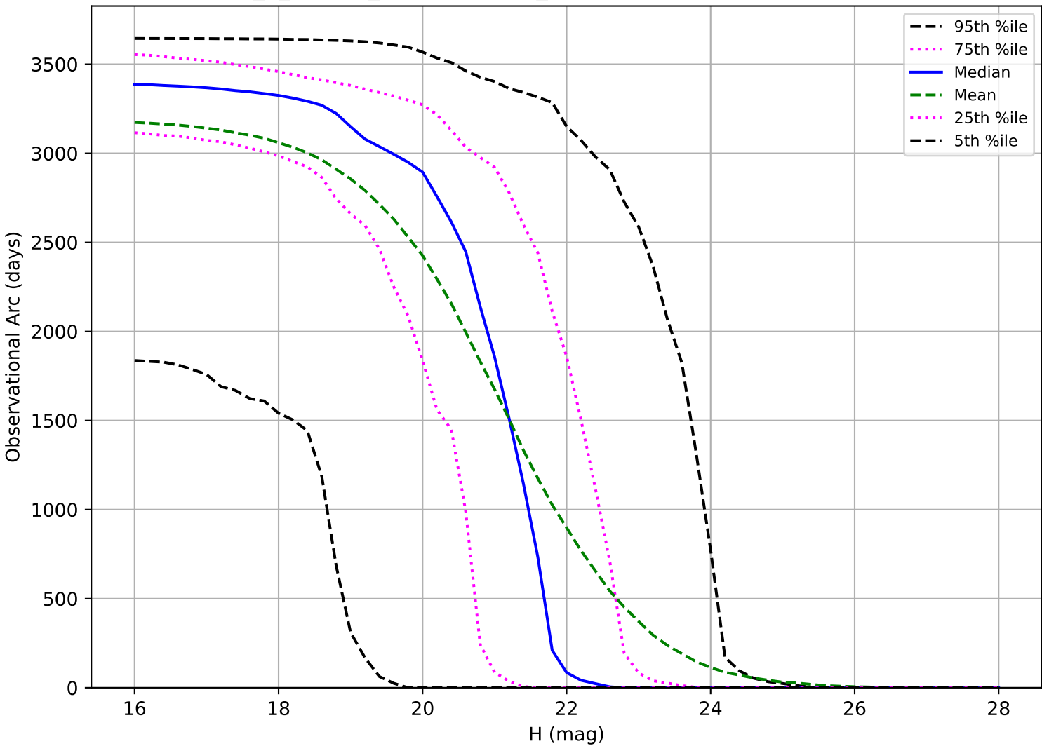
internal_u_expt38_nscale1.5v3.4_10yrs: Observational Arc Length NEO
