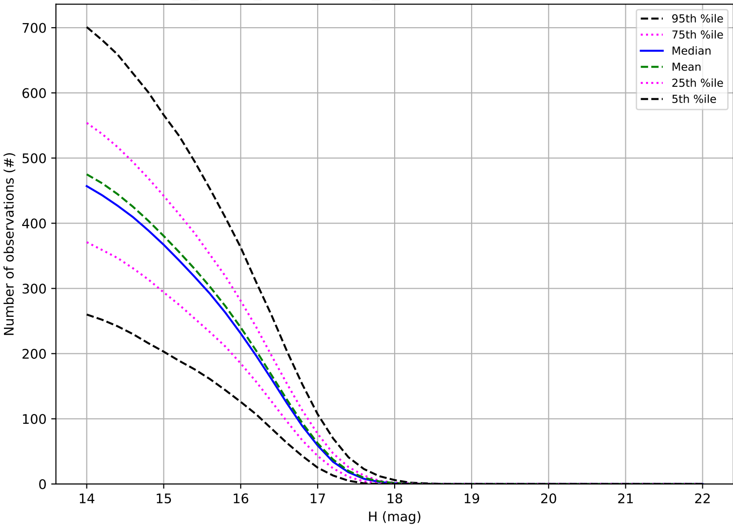
internal_u_expt38_nscale1.5v3.4_10yrs: Number of observations Trojan
