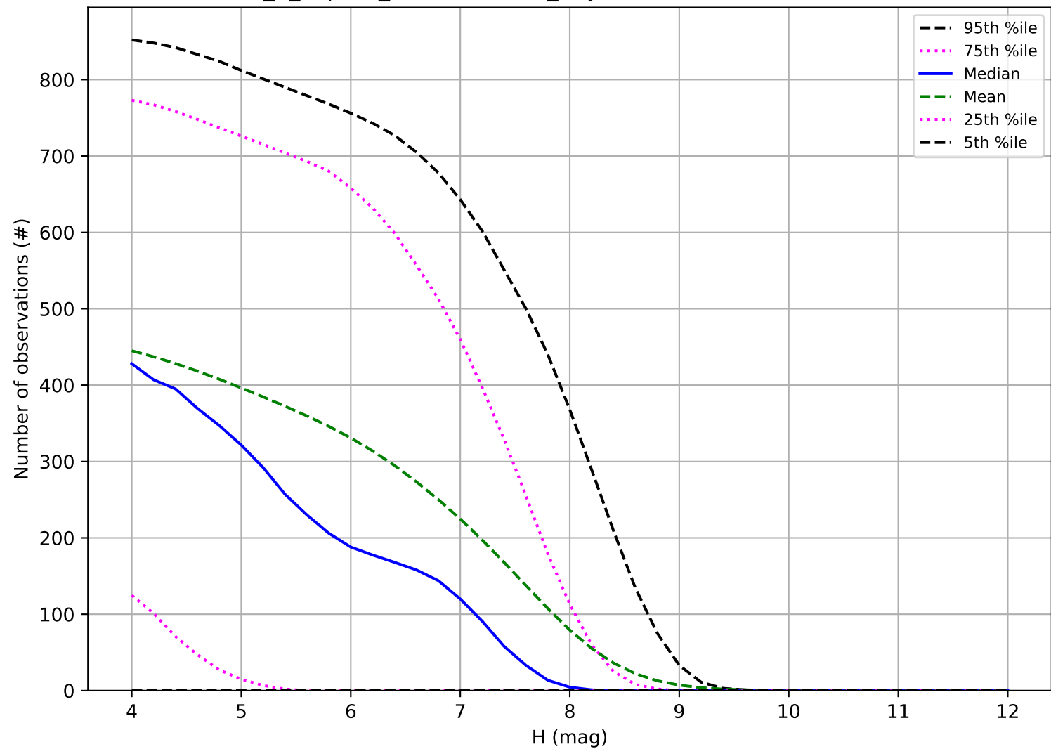
internal_u_expt38_nscale1.5v3.4_10yrs: Number of observations TNO
