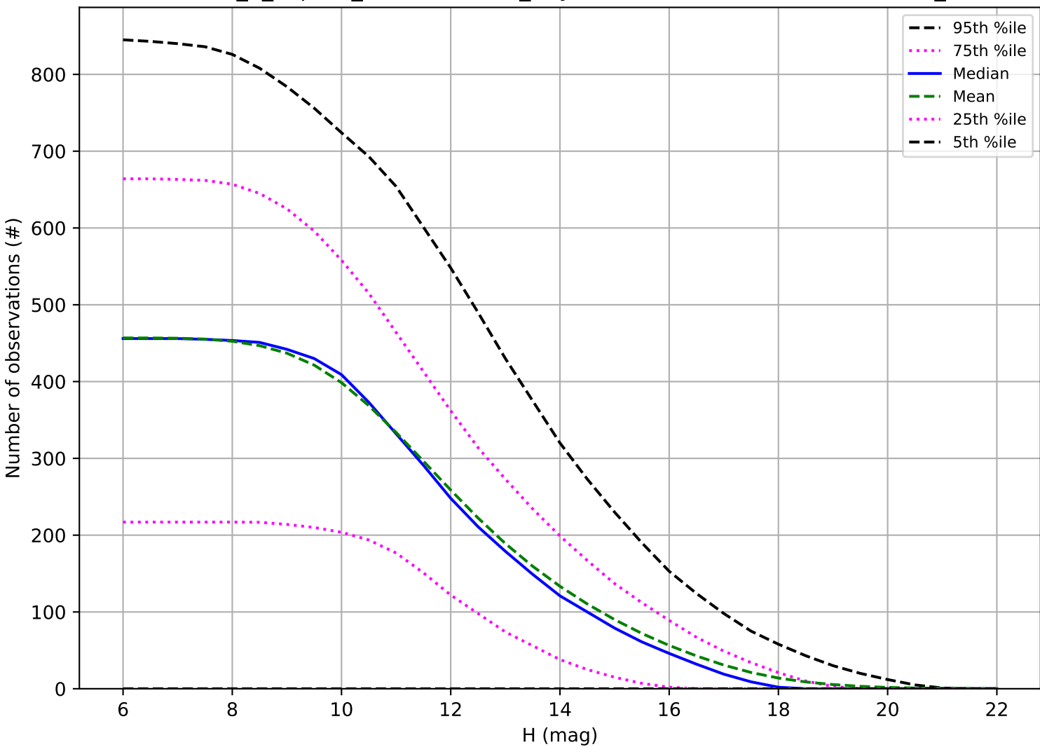
internal_u_expt38_nscale1.5v3.4_10yrs: Number of observations OCC_r5
