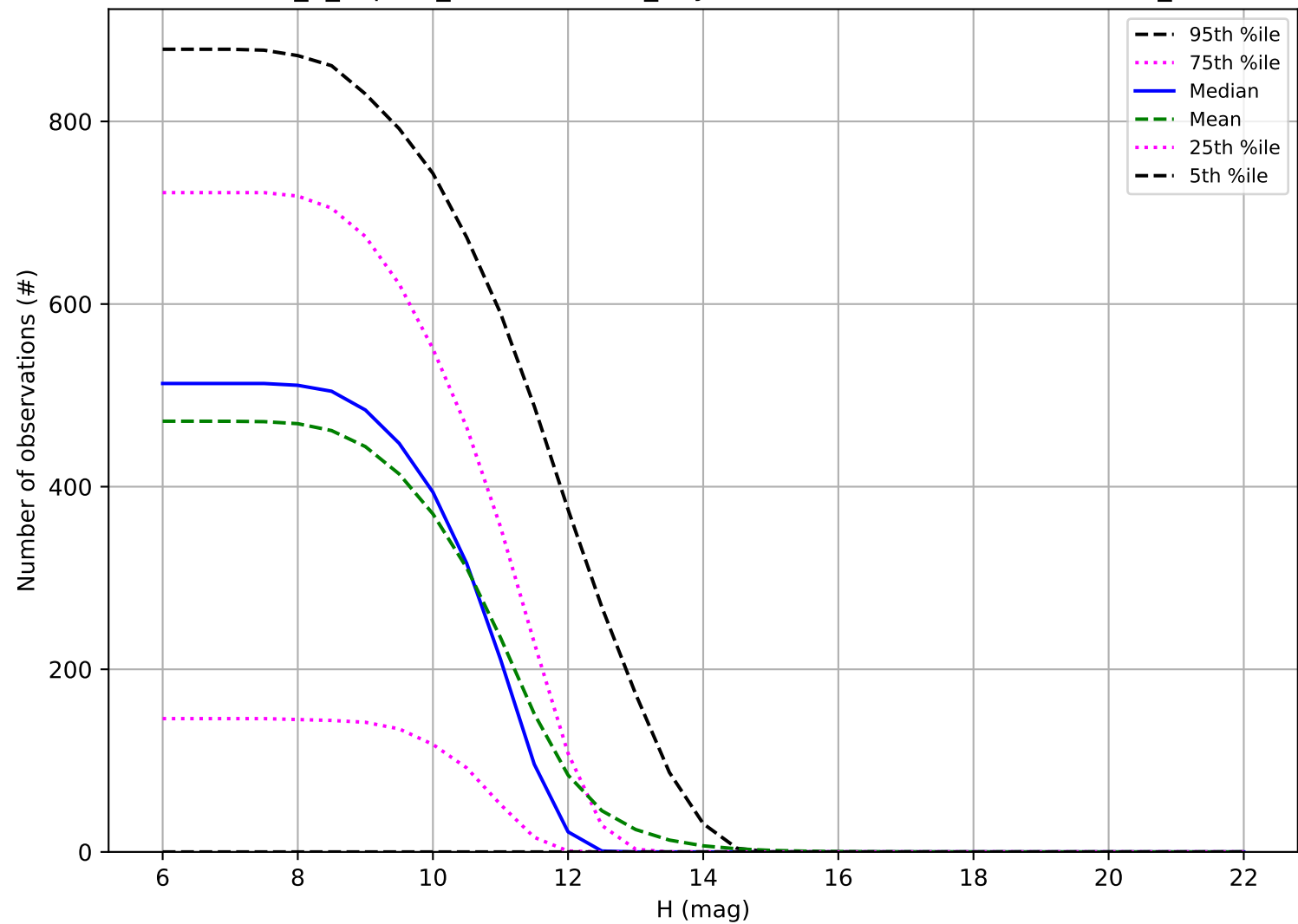
internal_u_expt38_nscale1.5v3.4_10yrs: Number of observations OCC_r20
