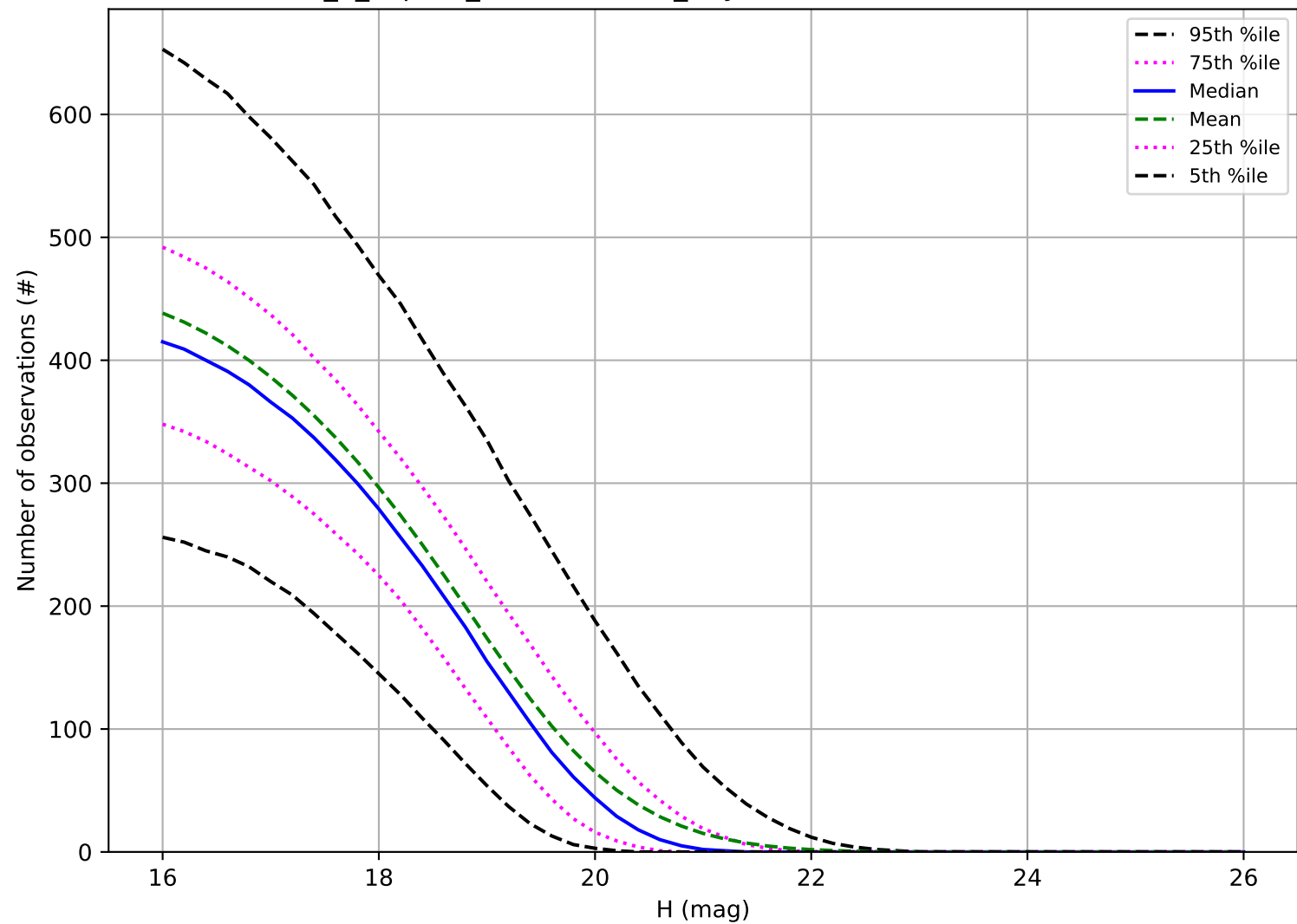
internal_u_expt38_nscale1.5v3.4_10yrs: Number of observations MBA
