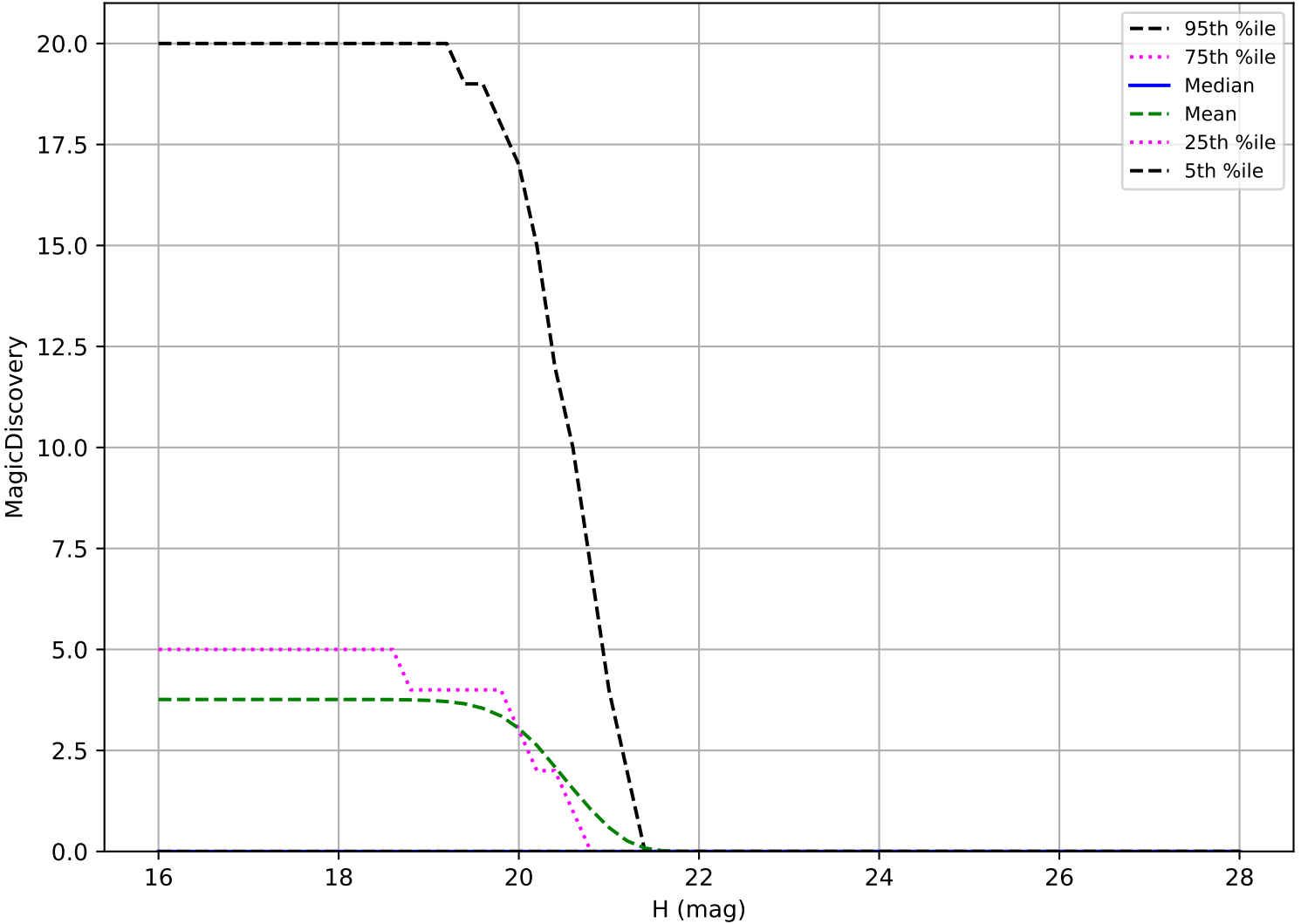
internal_u_expt38_nscale1.5v3.4_10yrs: Vatira 6 detections in 60 nights detection loss
