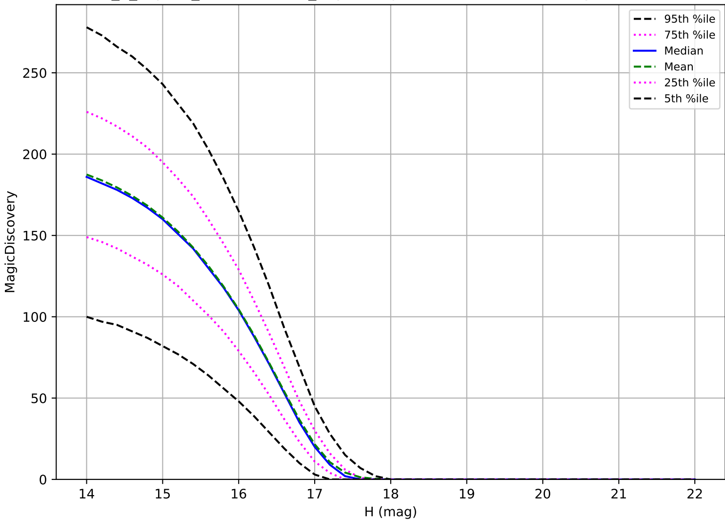
internal_u_expt38_nscale1.5v3.4_10yrs: Trojan 6 detections in 60 nights detection loss
