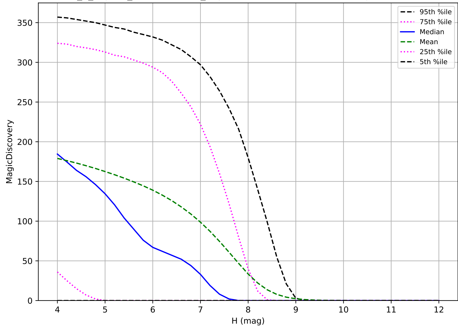
internal_u_expt38_nscale1.5v3.4_10yrs: TNO 6 detections in 60 nights detection loss
