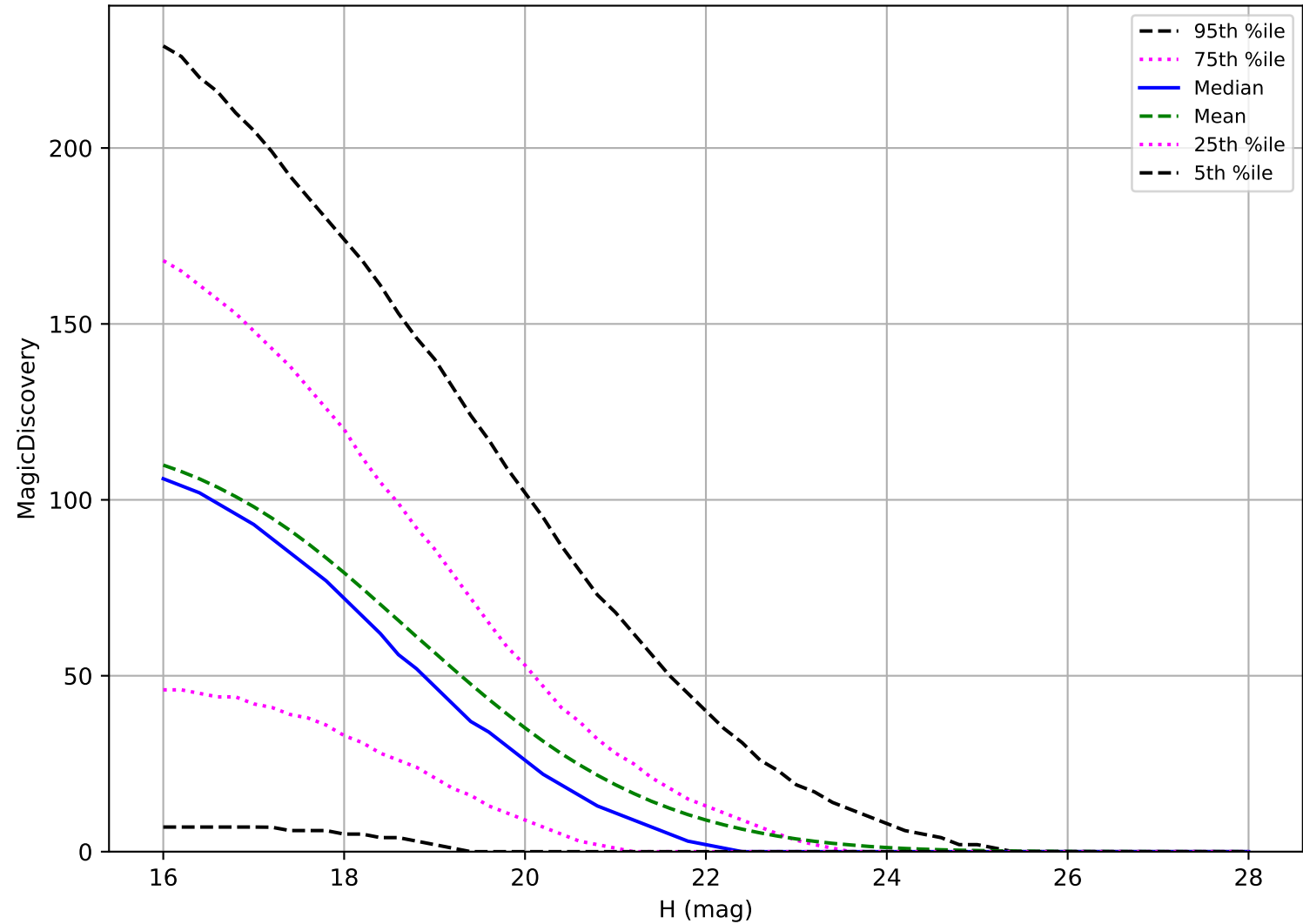
internal_u_expt38_nscale1.5v3.4_10yrs: PHA 6 detections in 60 nights detection loss
