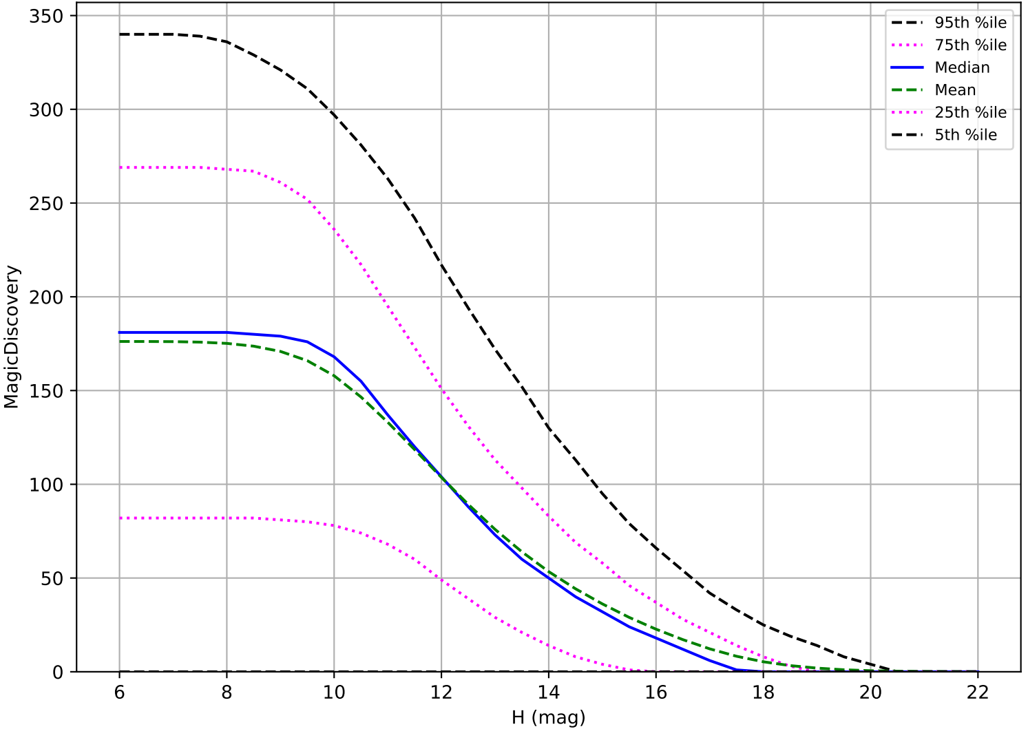
internal_u_expt38_nscale1.5v3.4_10yrs: OCC_r5 6 detections in 60 nights detection loss
