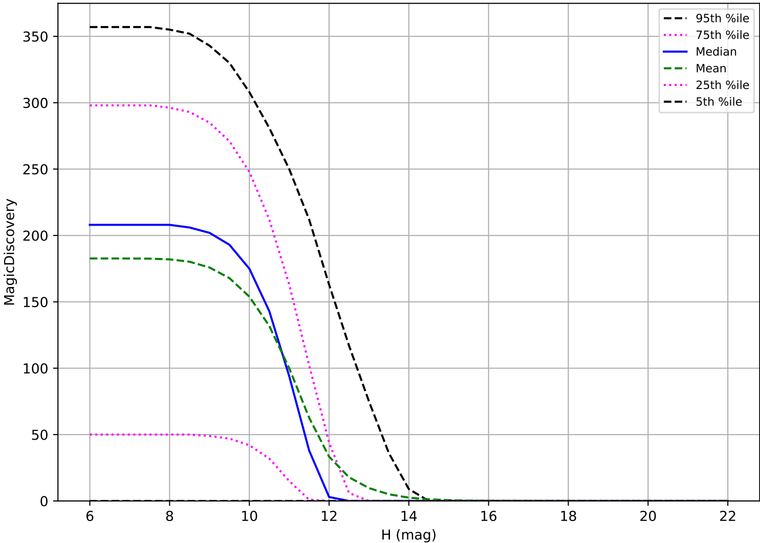
internal_u_expt38_nscale1.5v3.4_10yrs: OCC_r20 6 detections in 60 nights detection loss
