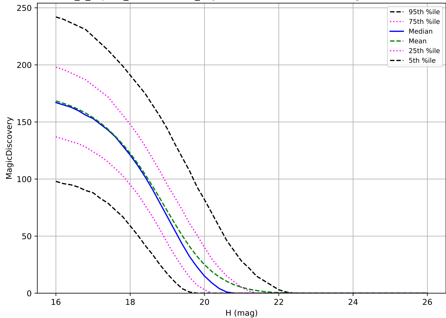
internal_u_expt38_nscale1.5v3.4_10yrs: MBA 6 detections in 60 nights detection loss
