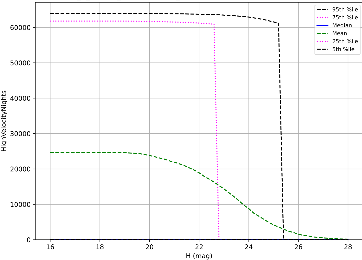
internal_u_expt38_nscale1.5v3.4_10yrs: PHA High velocity pair detection loss
