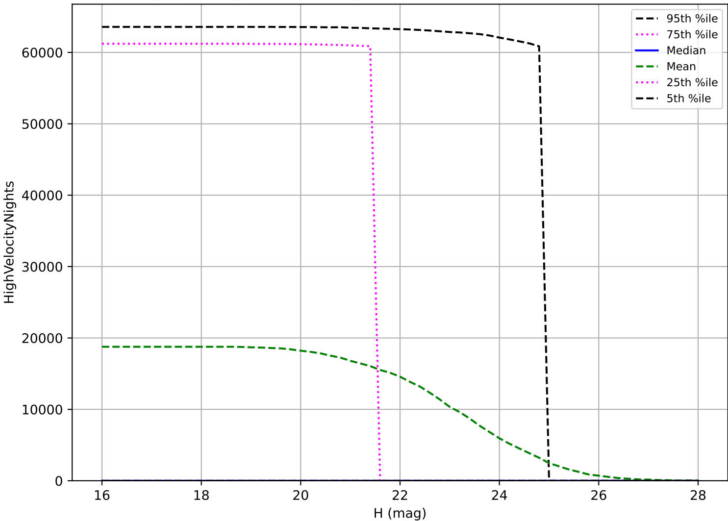
internal_u_expt38_nscale1.5v3.4_10yrs: NEO High velocity pair detection loss
