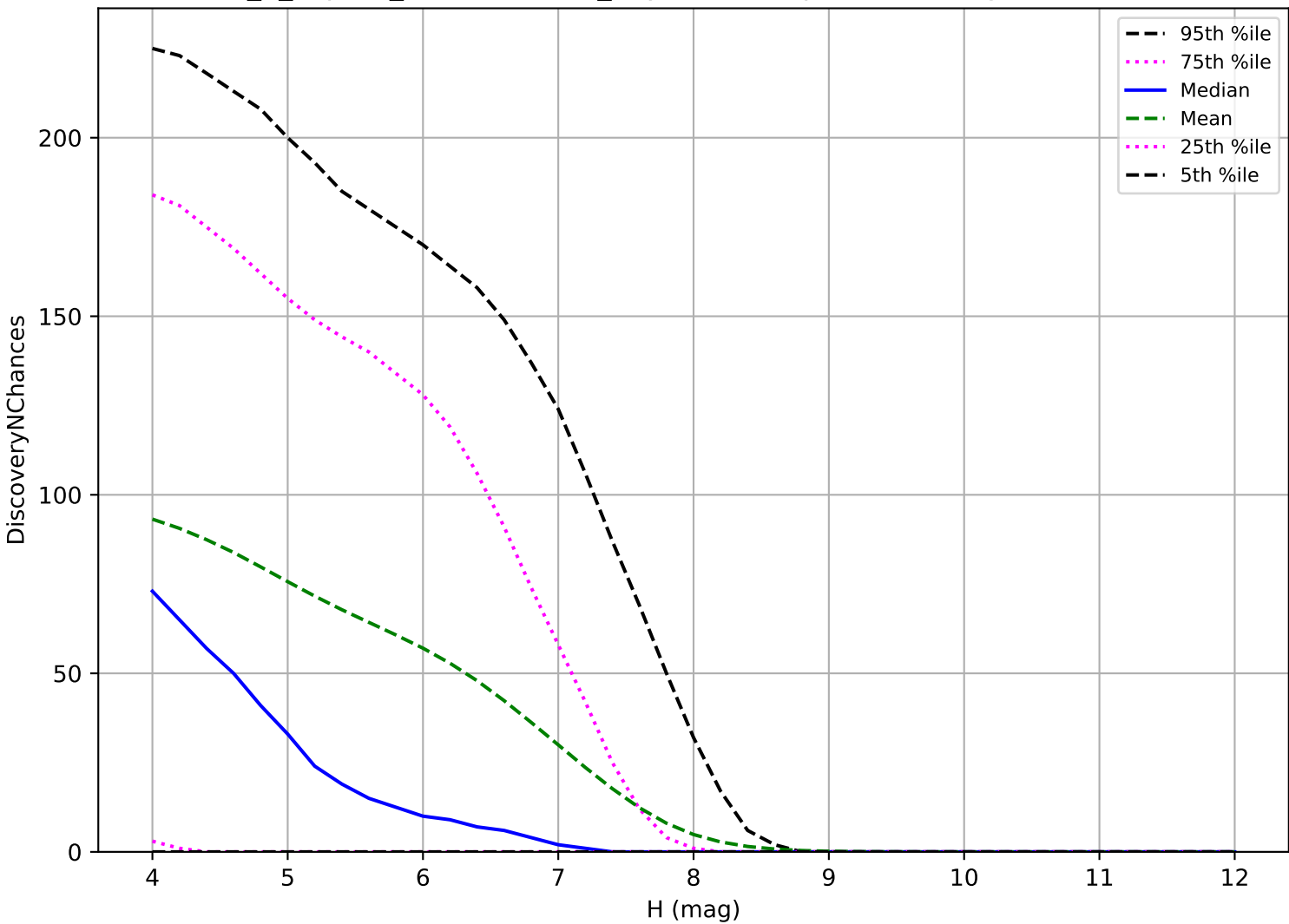
internal_u_expt38_nscale1.5v3.4_10yrs: TNO 3 pairs in 15 nights detection loss
