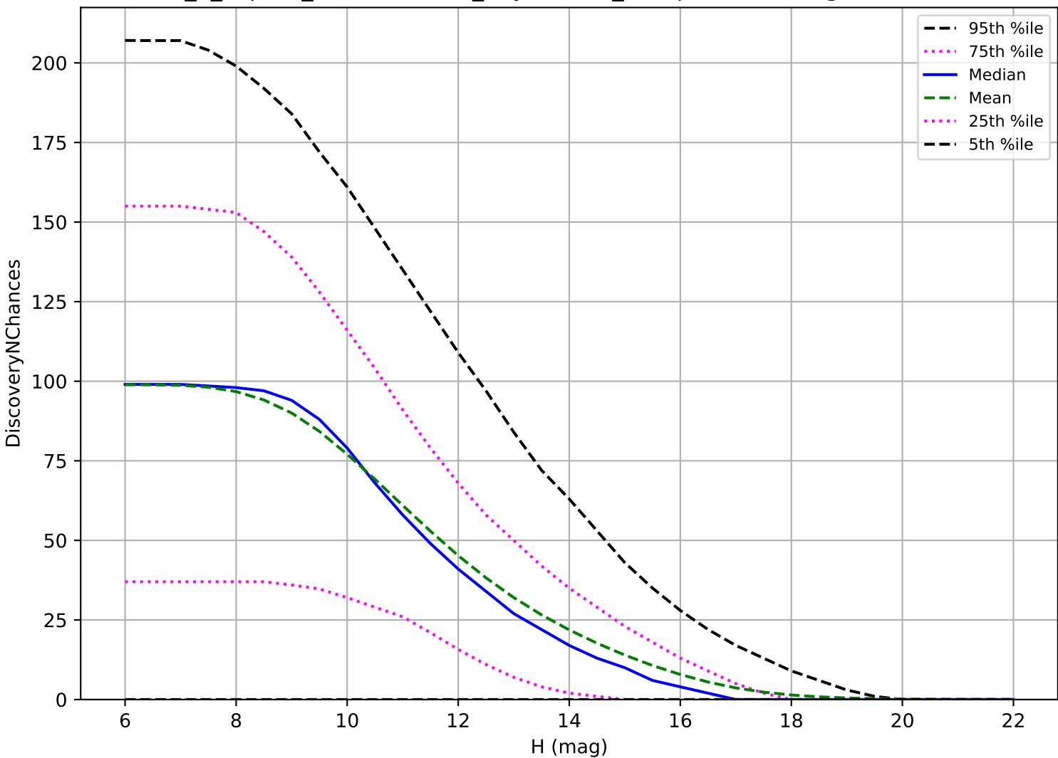
internal_u_expt38_nscale1.5v3.4_10yrs: OCC_r5 3 pairs in 15 nights detection loss
