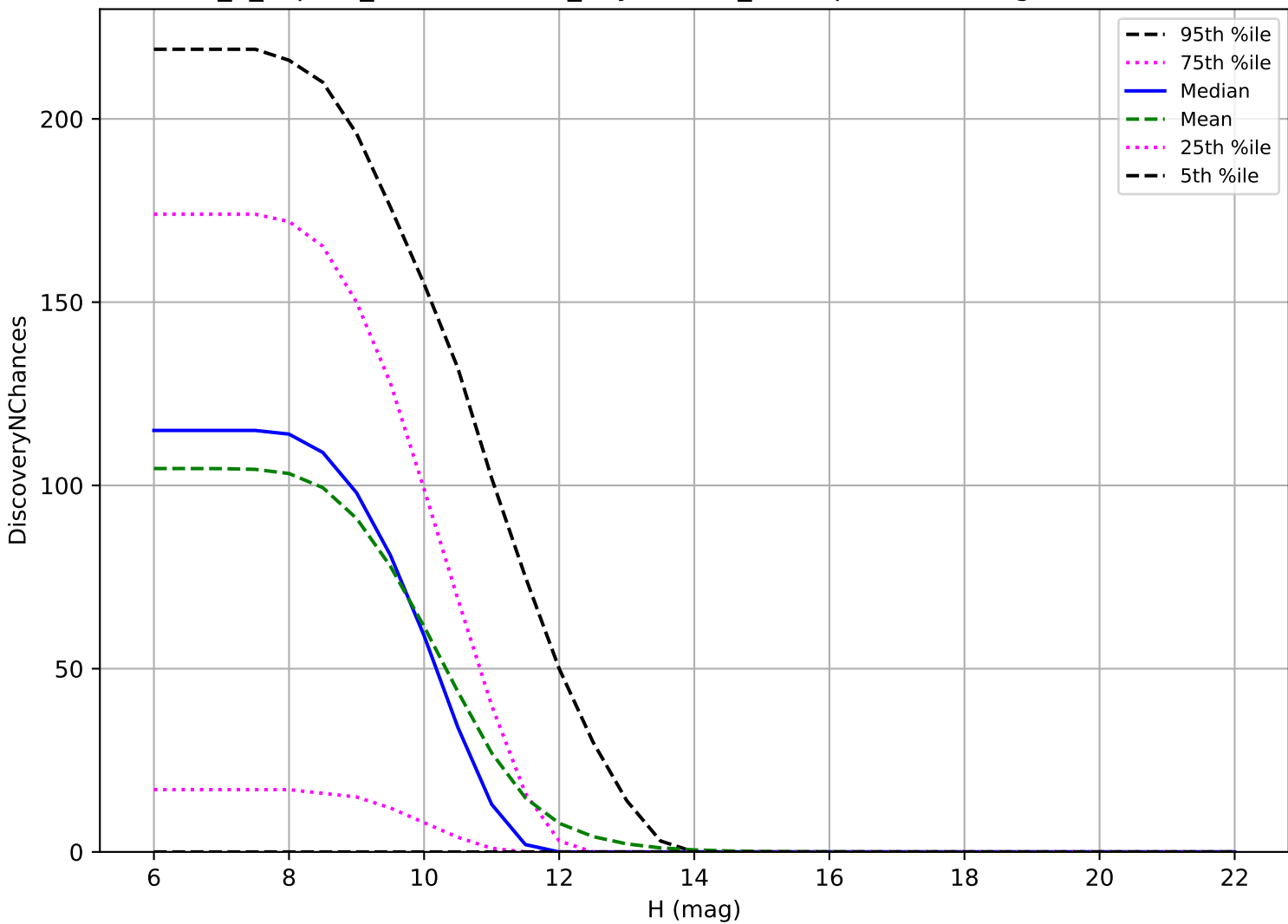
internal_u_expt38_nscale1.5v3.4_10yrs: OCC_r20 3 pairs in 15 nights detection loss
