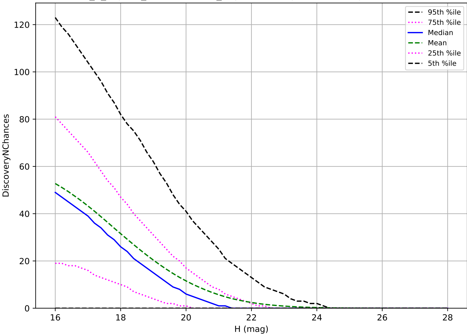
internal_u_expt38_nscale1.5v3.4_10yrs: NEO 3 pairs in 15 nights detection loss
