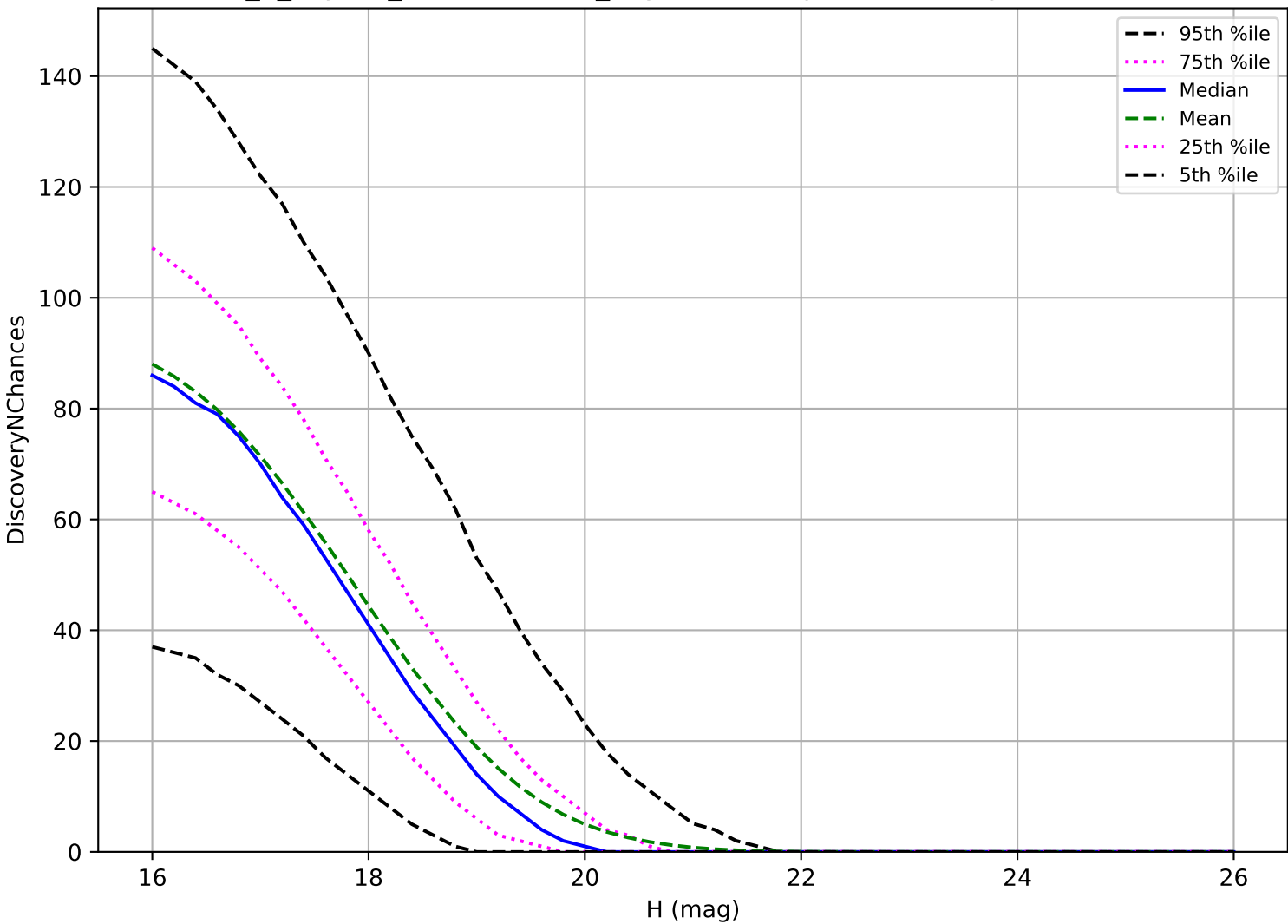
internal_u_expt38_nscale1.5v3.4_10yrs: MBA 3 pairs in 15 nights detection loss
