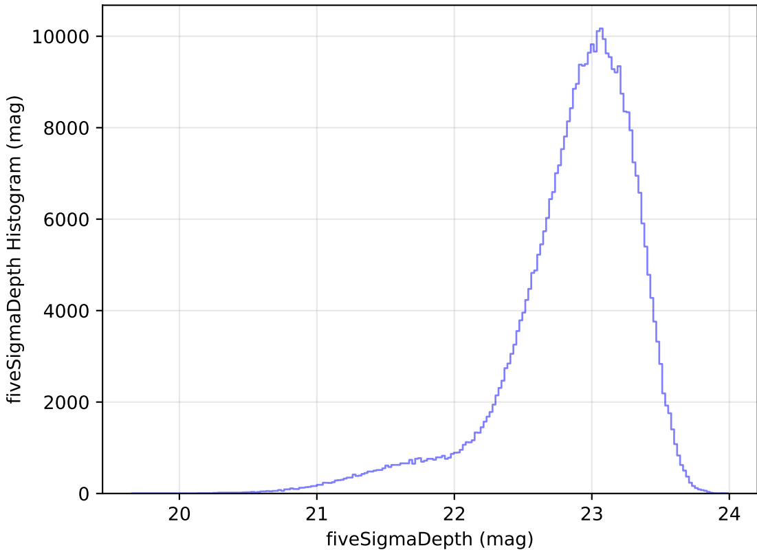
internal_u_expt38_nscale1.5v3.4_10yrs z: fiveSigmaDepth Histogram
