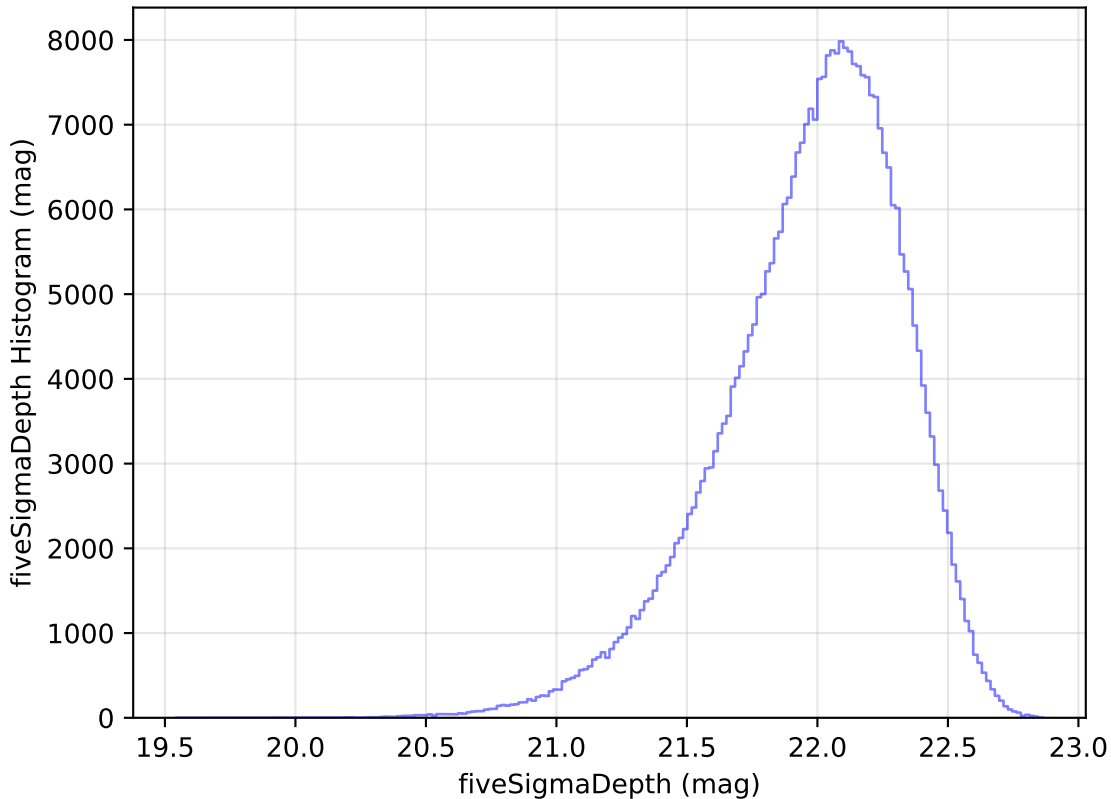
internal_u_expt38_nscale1.5v3.4_10yrs y: fiveSigmaDepth Histogram
