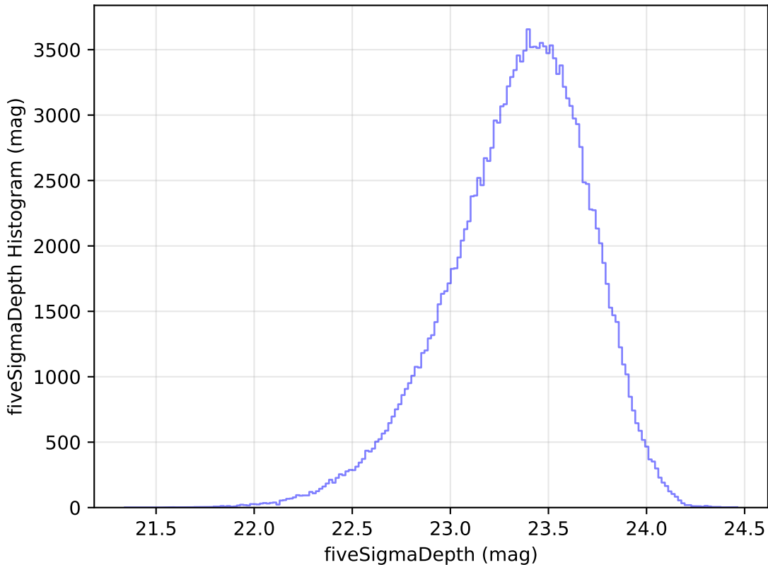
internal_u_expt38_nscale1.5v3.4_10yrs u: fiveSigmaDepth Histogram
