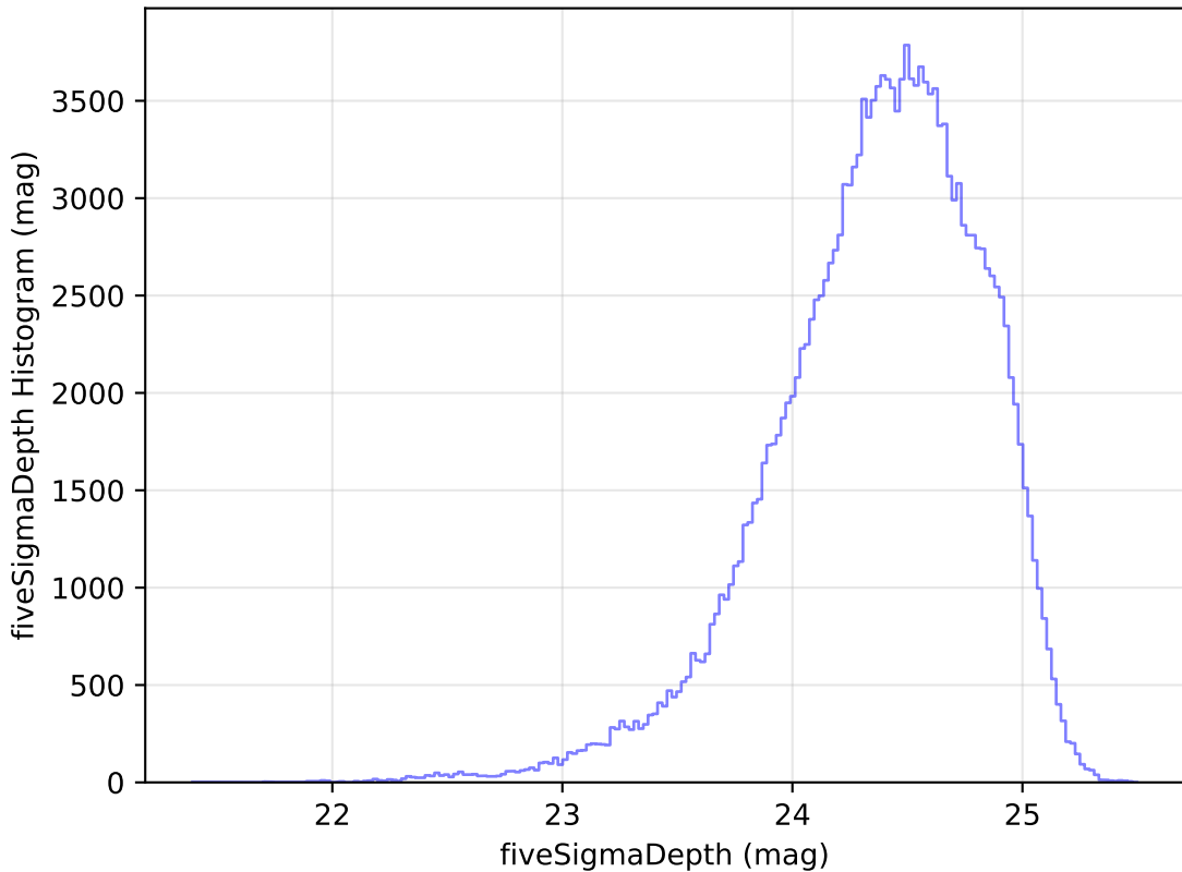
internal_u_expt38_nscale1.5v3.4_10yrs g: fiveSigmaDepth Histogram
