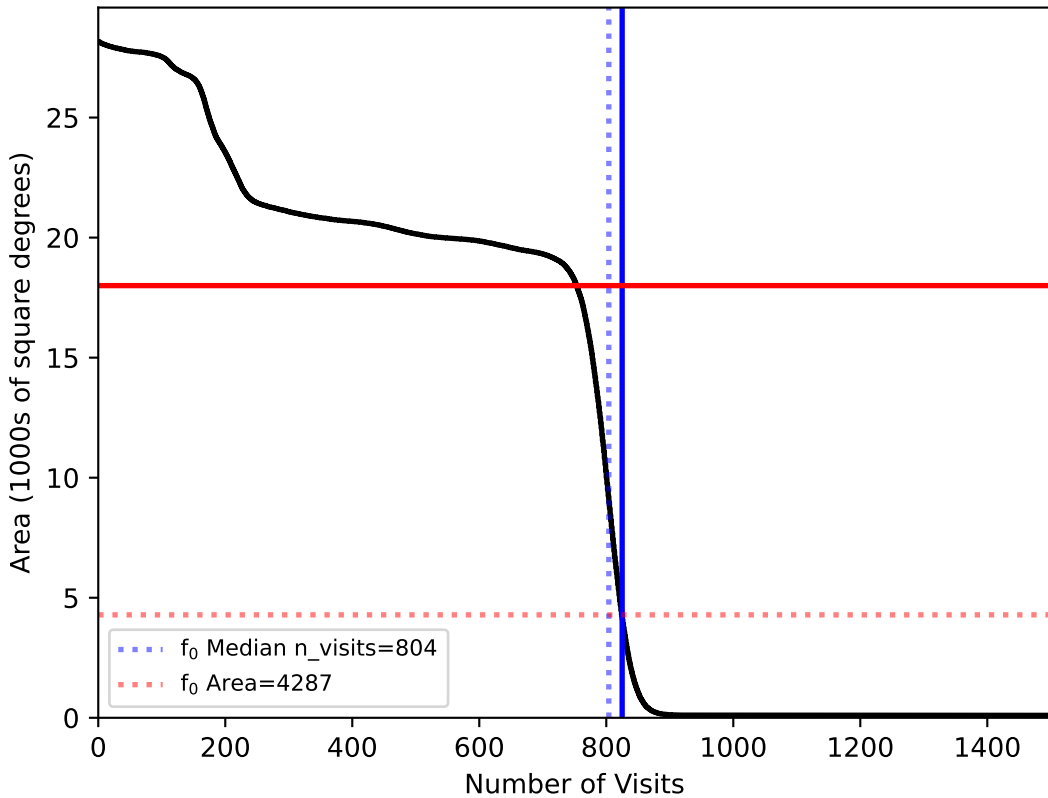
internal_u_expt38_nscale1.5v3.4_10yrs : fO
