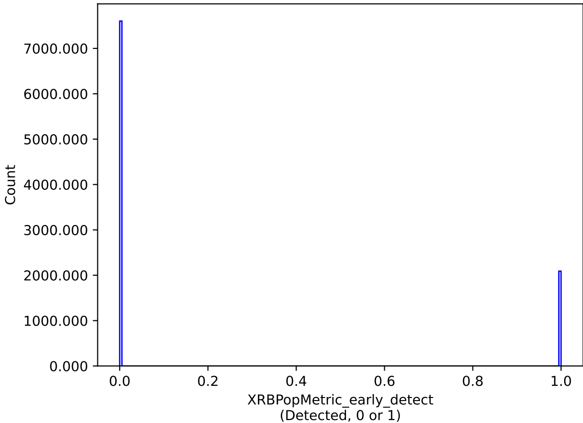
internal_u_expt38_nscale1.5v3.4_10yrs : XRBPoMetric_early_detect
