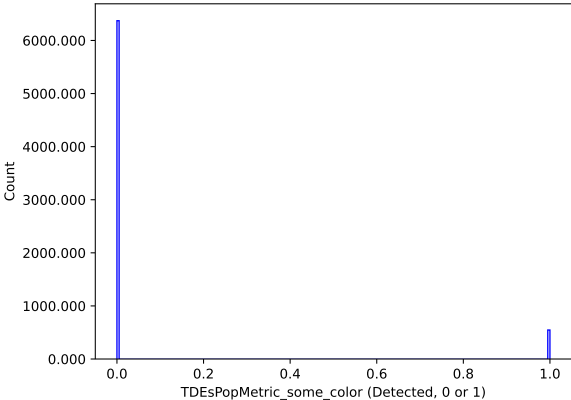
internal_u_expt38_nscale1.5v3.4_10yrs : TDEsPopMetric_some_color
