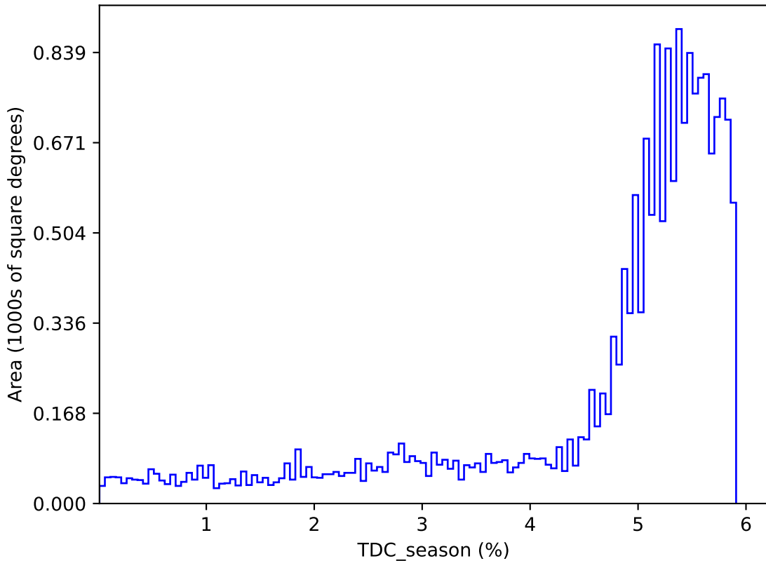
internal_u_expt38_nscale1.5v3.4_10yrs : TDC_season
